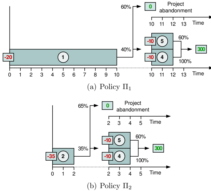
Figure 3: Policies with deterministic durations
