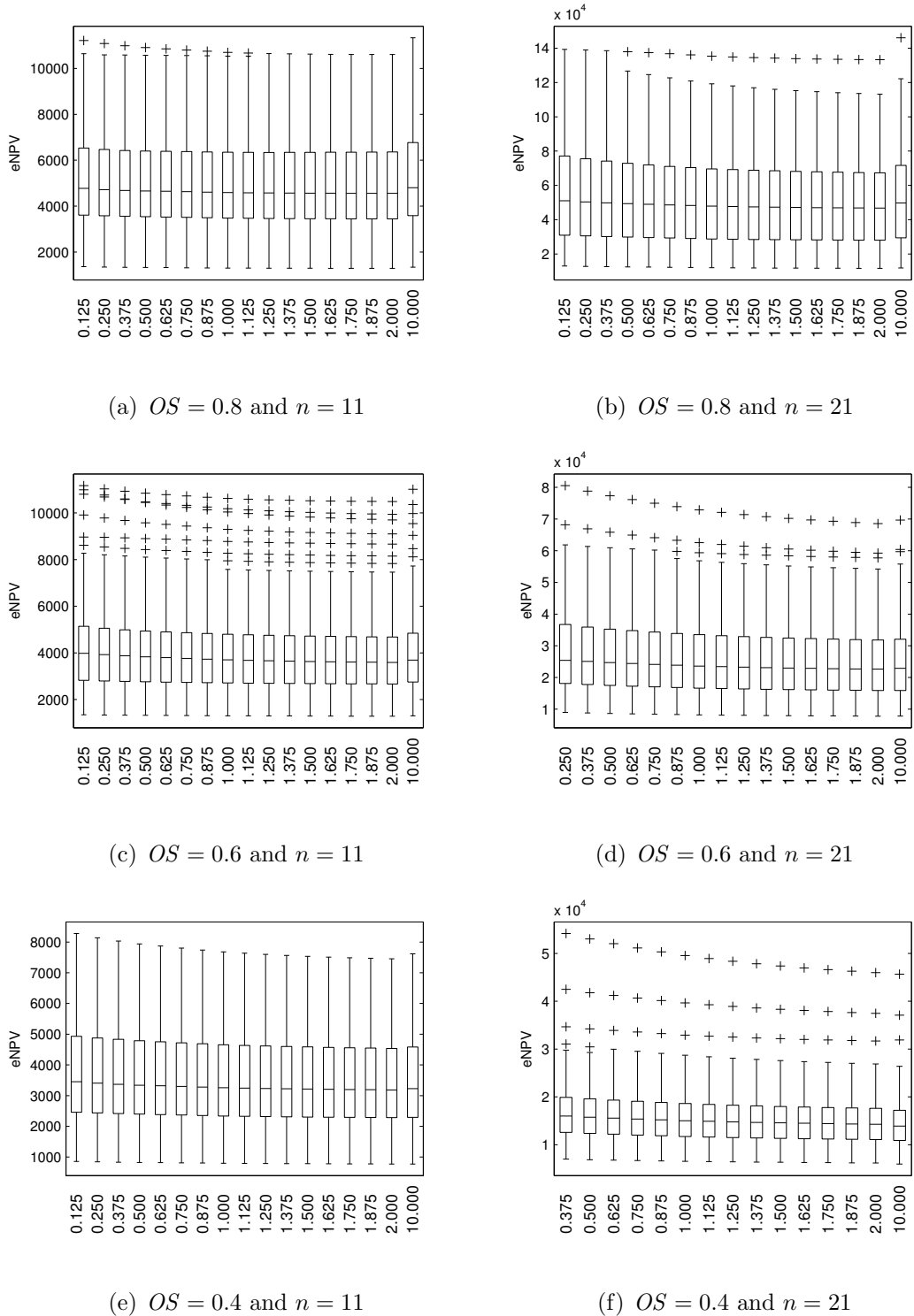
Figure 8: Boxplots of eNPV for different values of SCV , n and OS with r = 0.01
